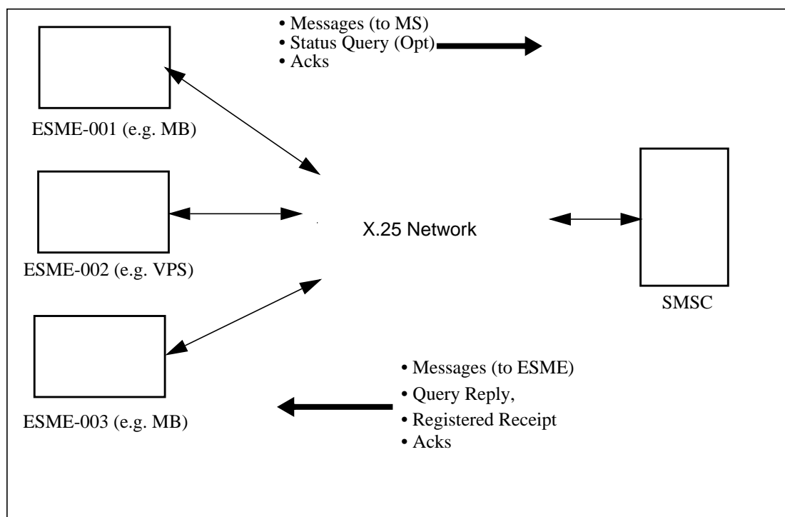
Figure 2-1: SMSC & ESME Interworking using X.25
