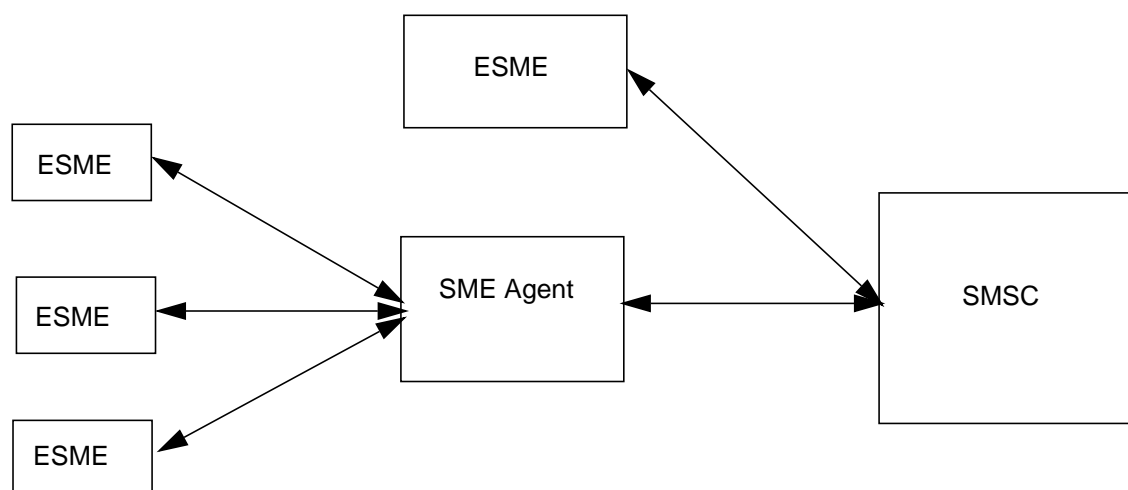
Figure 6-1: ESME/SME address routing to/from SMSC
