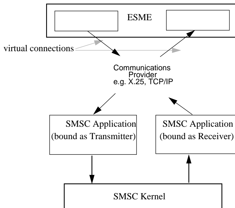
Figure 5-1: ESME/SMSC Communication
